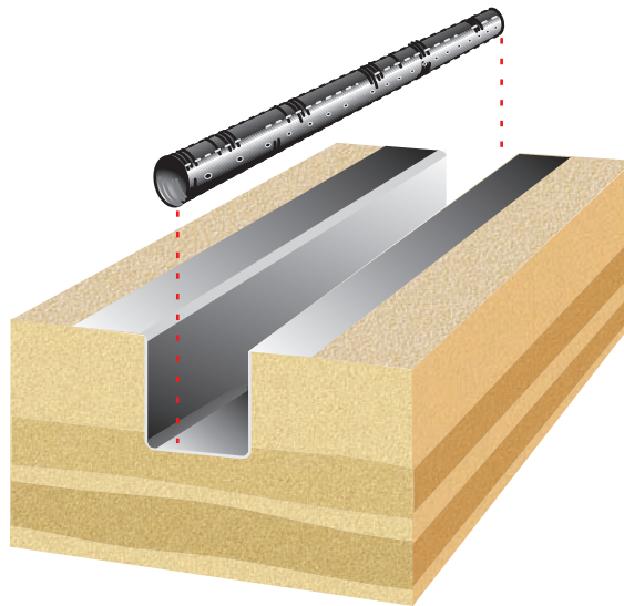
INSTALL FABRIC AND 4" PERFORATED PIPE
