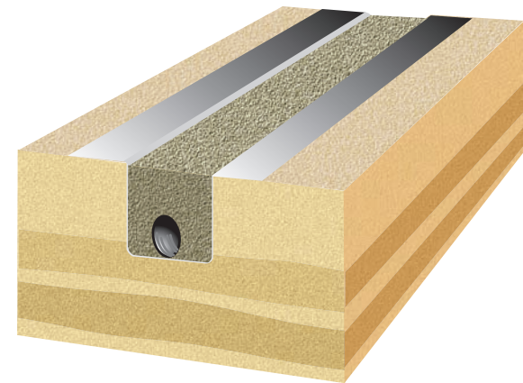
FILL WITH 3/4" ROCK
